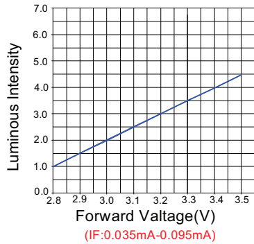
Luminous Intensity VS Forward Voltage
