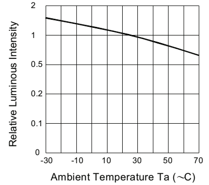
Relative Luminous Intensity Vs Ambient Temperature
