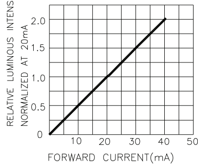
FORWARD CURRENT VS LUMINOUS INTENSITY
