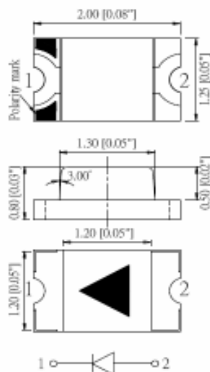
Package outlines
