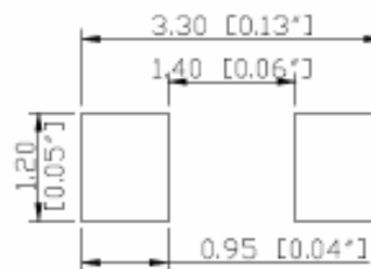
Recommend Pad Layout
